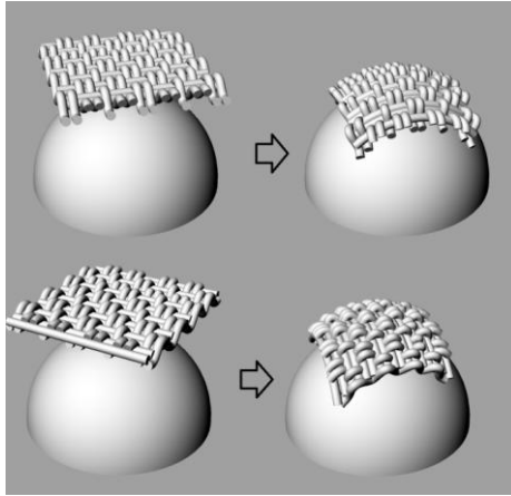
Figure 6. Mechanical simulation of draping process including a combined mechanical modeling of compression, bend, stretch, and shear shown from two different draping angles; considering geometry and materials selection simultaneously.
