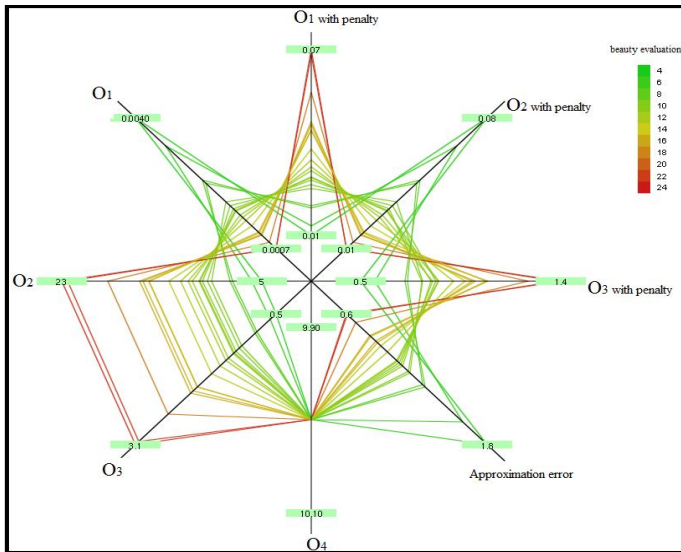
Figure 5. Case study; considering four objectives in addition to beauty evaluation function in a multi-dimensional graph [48]
