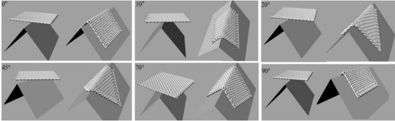
Figure 4. Draping simulation in textile composites [49], [50] considering a number of draping degrees
