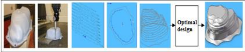
Figure 1. Shape optimization for complex geometries; the workflow
